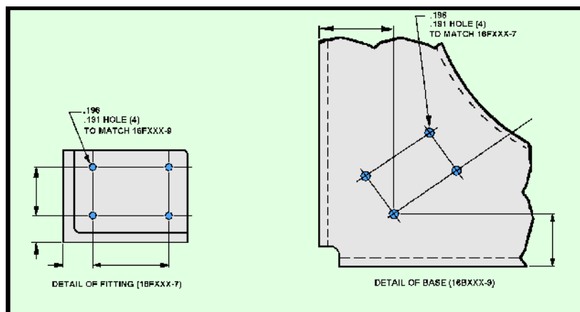
Figure 13. Example of "To Match" hole patterns as defined on engineering drawings.
