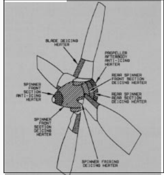
The propeller contains both anti-icing and deicing elements.
