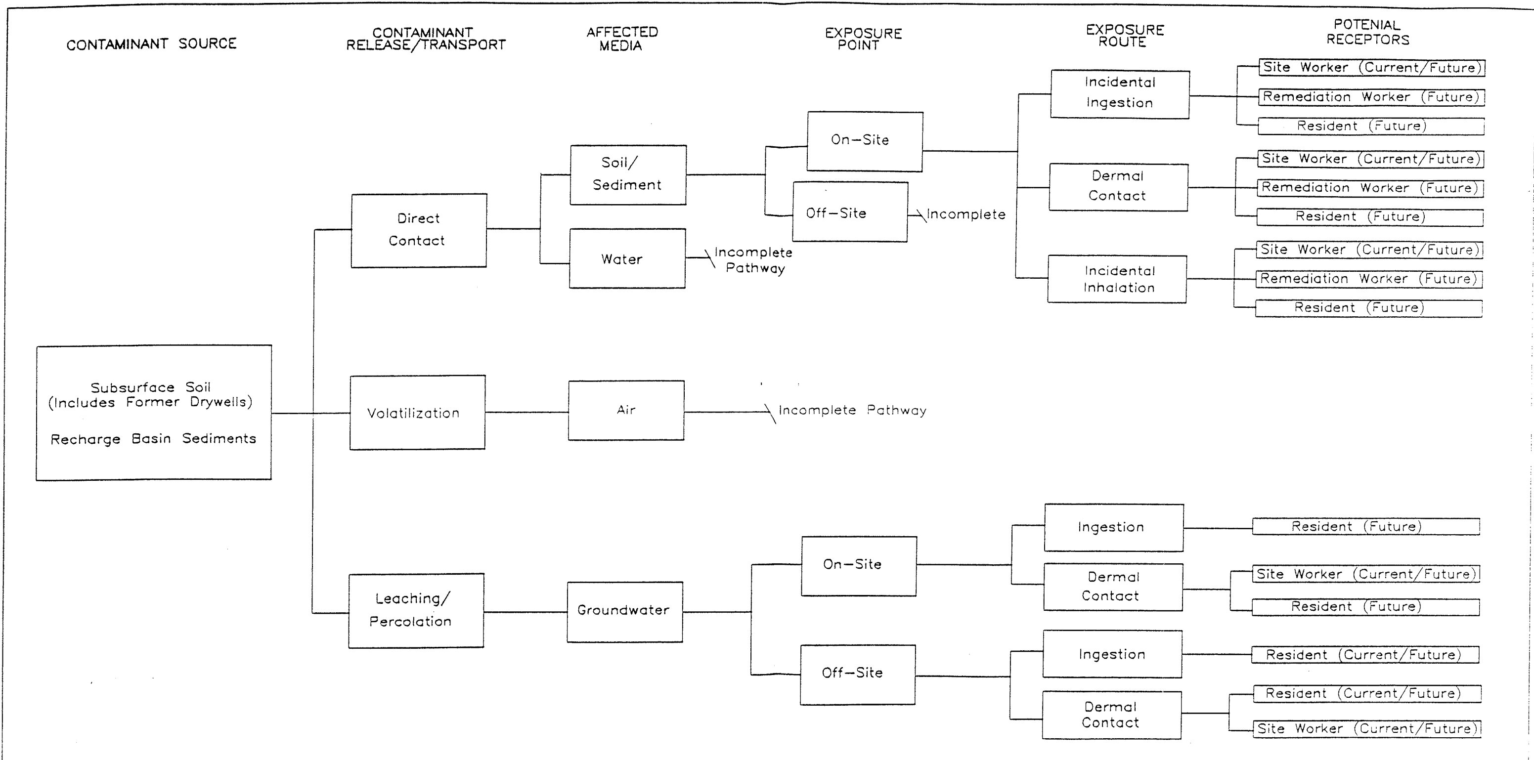
FIGURE 4-1 SUMMARY OF EXPOSURE PATHWAYS LOCKHEED MARTIN GREAT NECK, NEW YORK
